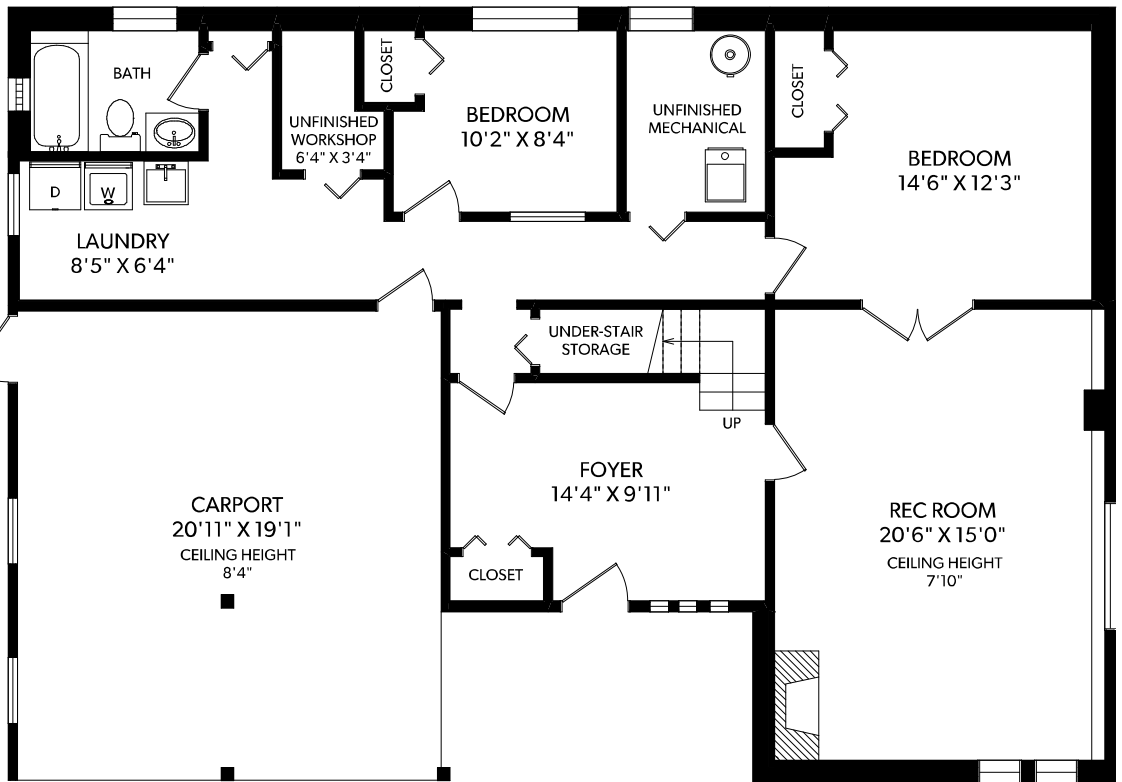
LOWER FLOOR
